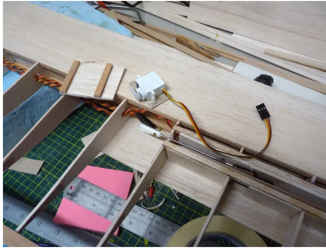
Left: Basic airbrake assembly. | Right: Airbrake installed in the wing.
