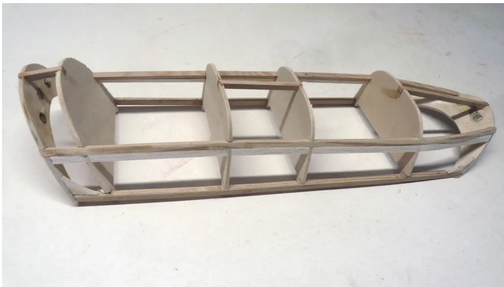
The hatch, ready for sheeting.
