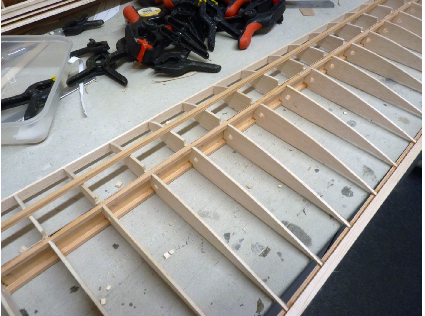
01: With the slots cut out, the sub spar is ready to glue in place.
