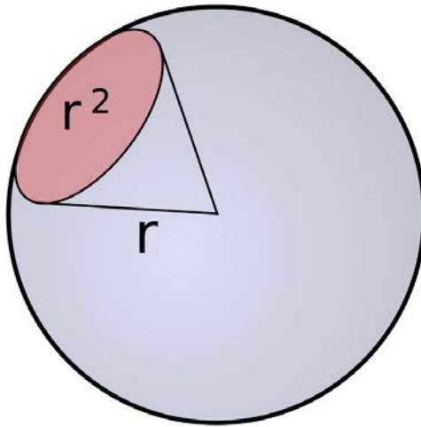
Figure 2: The cone is one steradian. (credit: Wikimedia under CC BY-SA 3.0)
