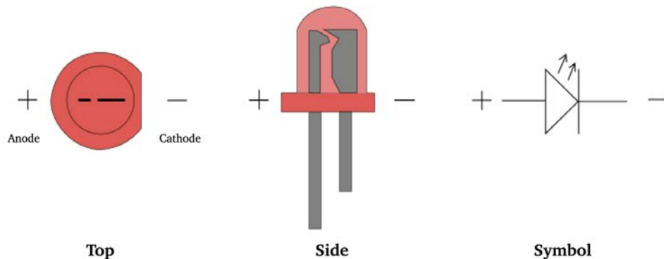
Picture 1: What a bare LED looks like and a common circuit symbol.
