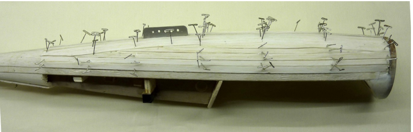
Filled and sanded with two coats of Eze-Kote , before glassing:
