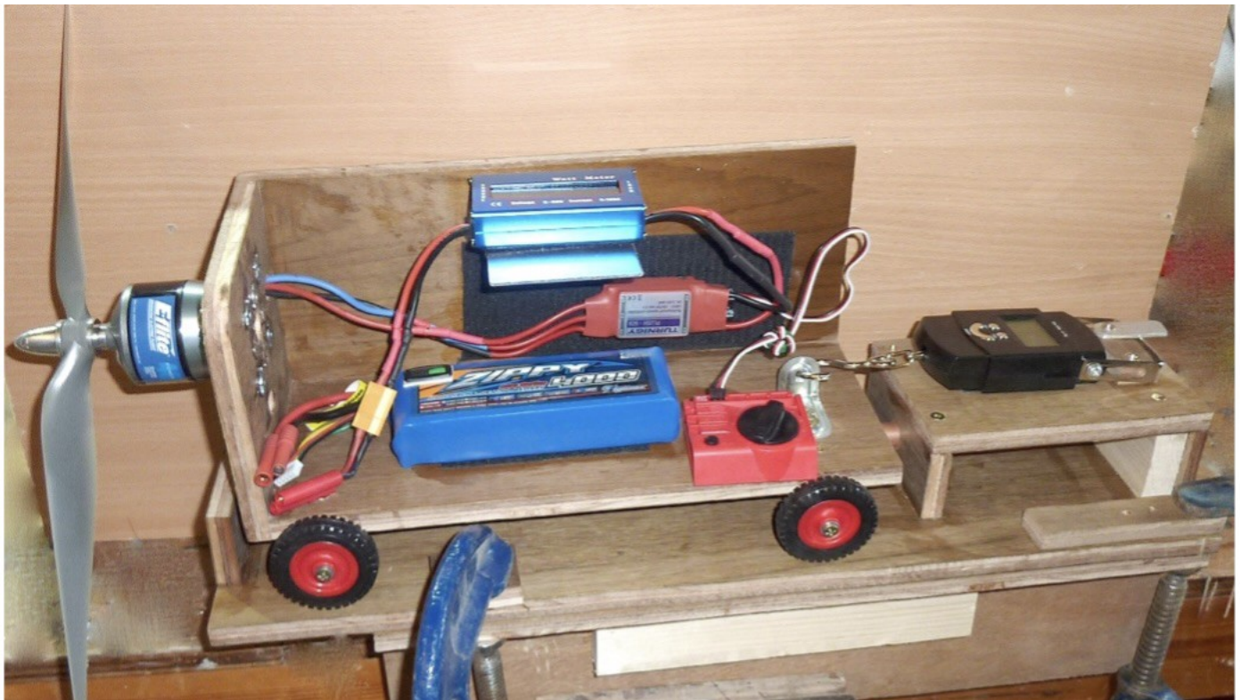
Picture 1: Test rig for motors employing the Martin Phillips design featured in RCM&E. (credit: Peter Scott)
