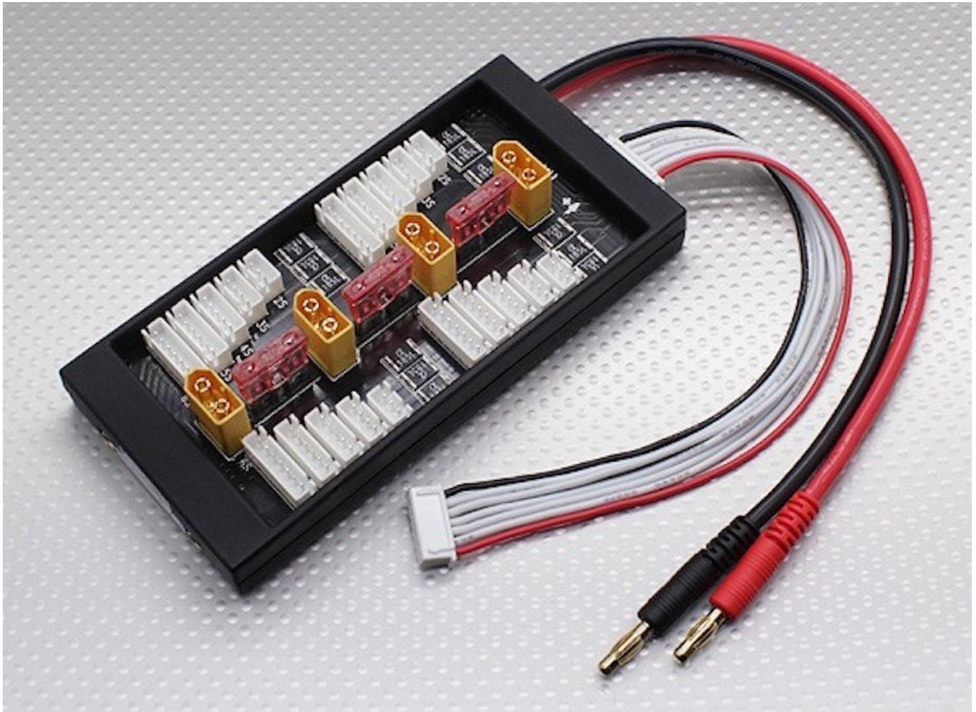
Picture 2: HobbyKing parallel charge board. (image: HobbyKing)
