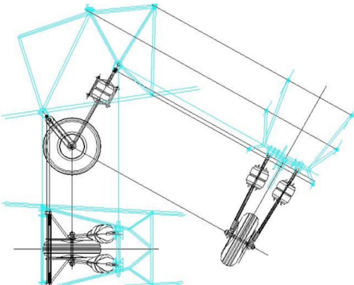
Drawing 16: Main landing gear assembly
