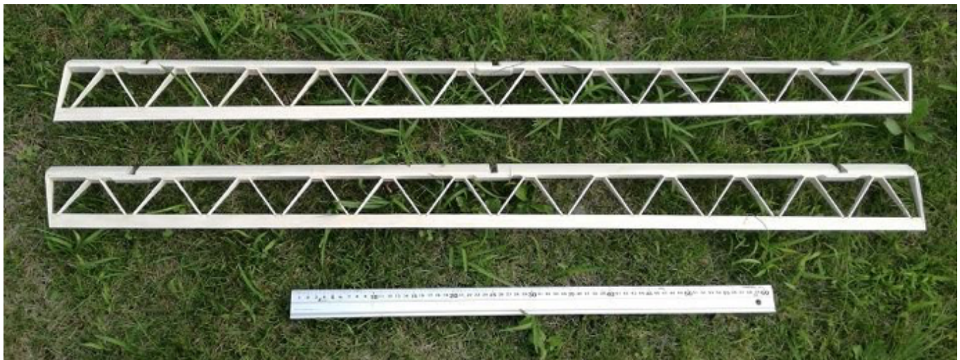
Photo 35: Finished aileron assembly
