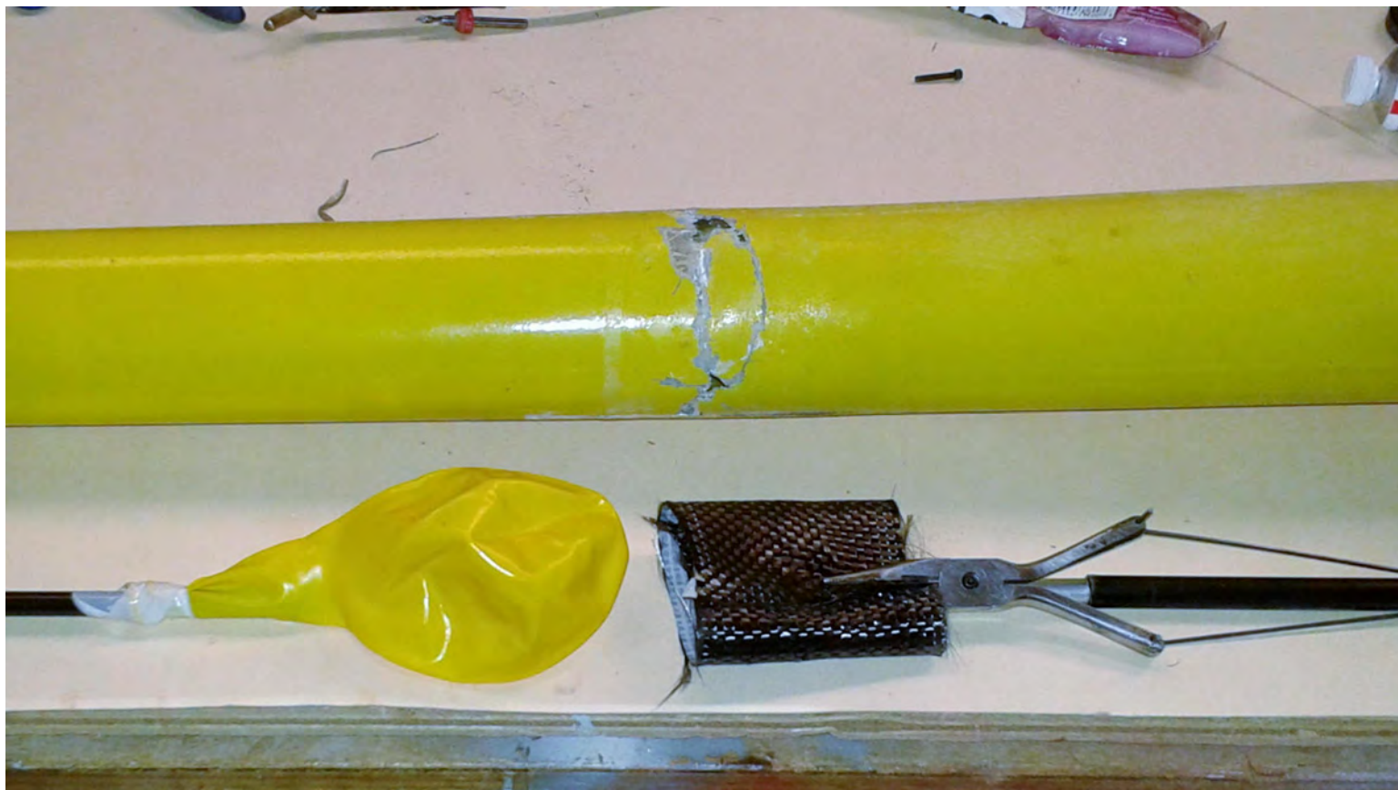
Photo 1: The Extra Long Reach Pliers in action, fixing a wayward Aquila XL fuselage.
