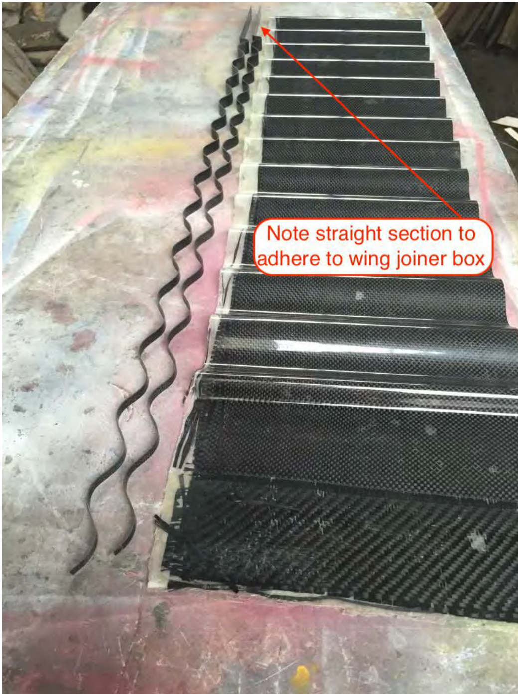
Photo 4: A whole sheet of early spars. Later the carbon was reduced and carefully oriented for optimum strength. (image: James Hammond)
