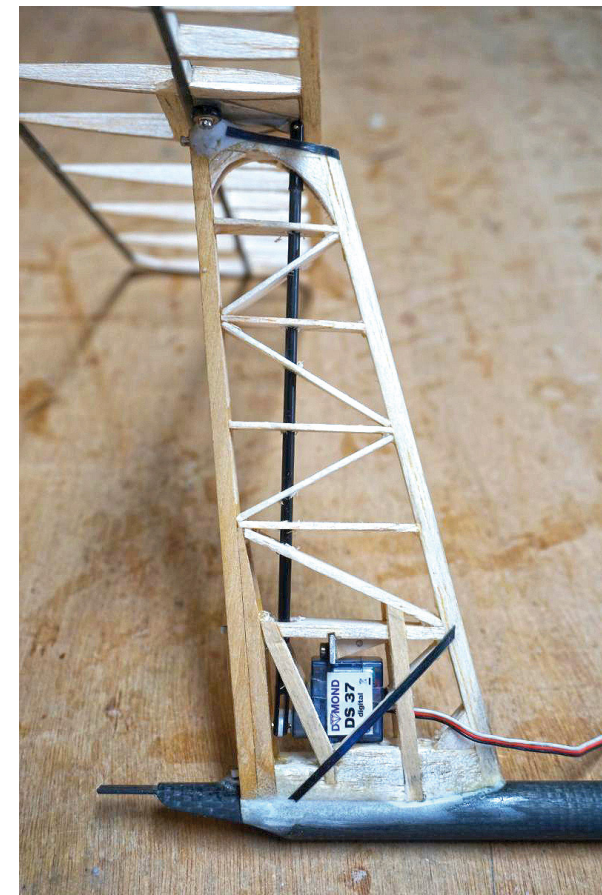
Vertical fin showing servo location and carbon rod elevator transmission.
