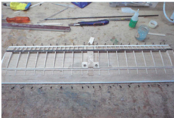
From top to bottom and left to right: wing building sequence and central panel building
