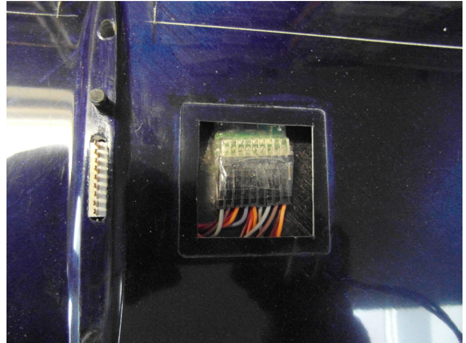
The 8-channel FRsky SBUS is mounted in the wing and drives eight servos - ailerons, flaps, leading edge flaps.
