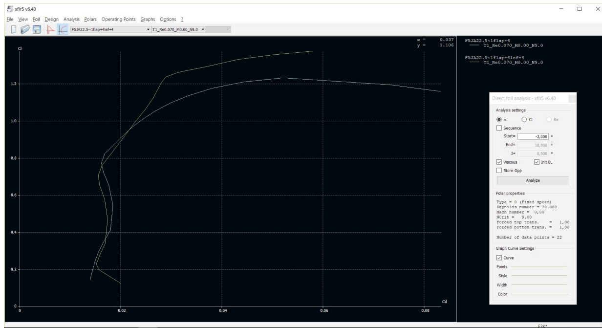
Polar comparison of airfoil with flaps deflected and with flaps and leading edge flaps deflected. Notice changes in the upper part of the curves.
