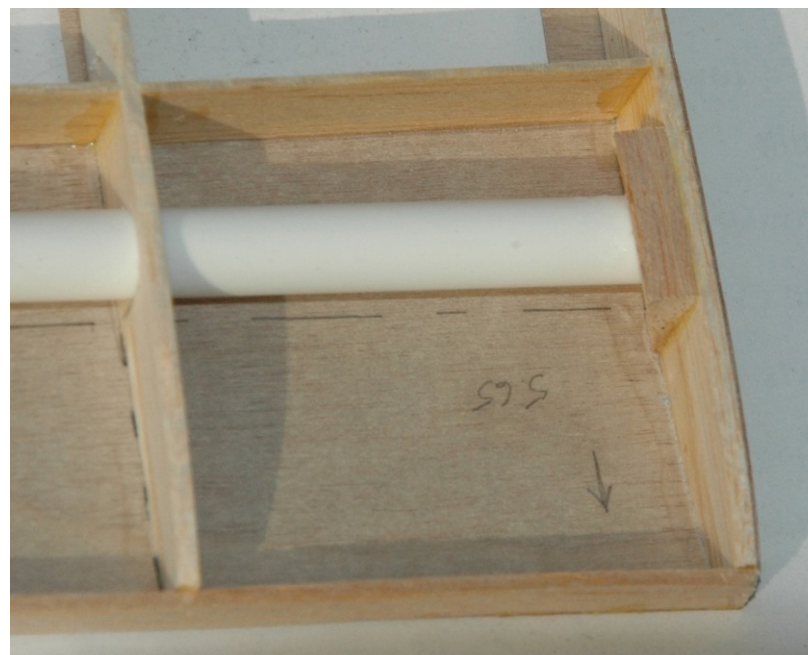
Figure T1: Tail root rib with control horn wedge.
