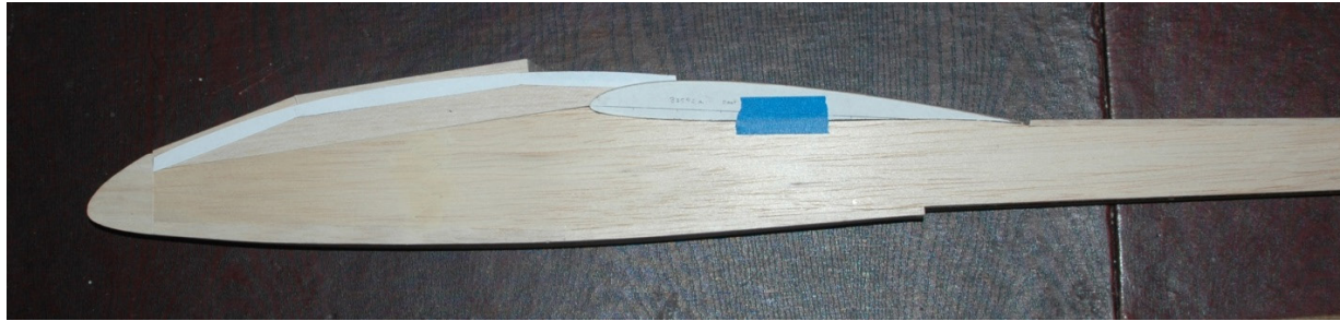
Figure F15: Marking the hatch cover for wing fit
