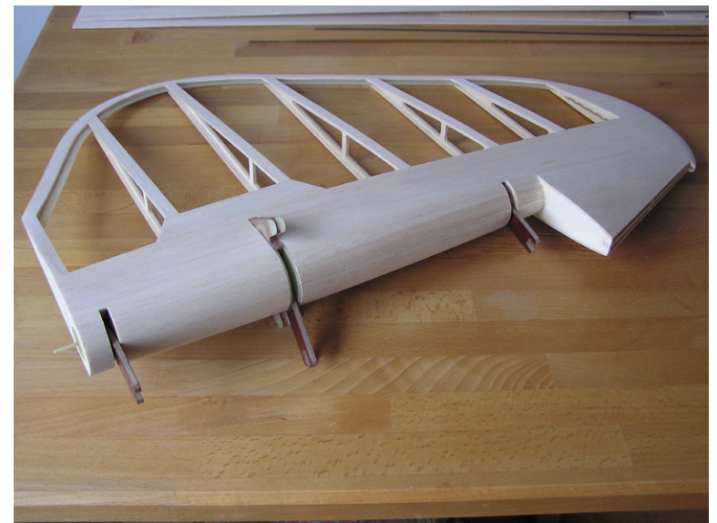
Rudder with skin made of balsa, pivots and drive
