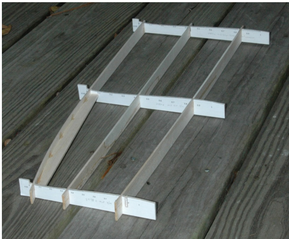
Figure W21: Tip panel jig
