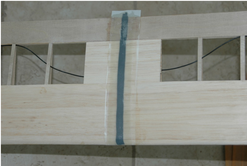
Figure F9: Reinforcing the wing panel joint with carbon fiber tape, fiberglass and peel ply.
