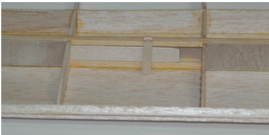
Figure W12: Tip Joiner in the wing spar with the spacer wedge in front
