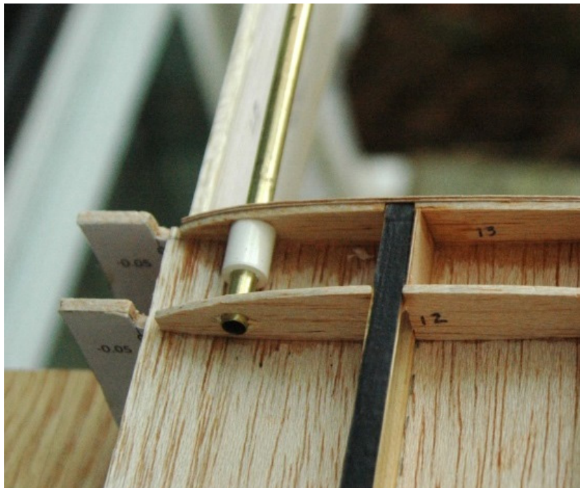
Figure W11: Installation of the wing tip locating pin bushings — carbon spar caps are optional
