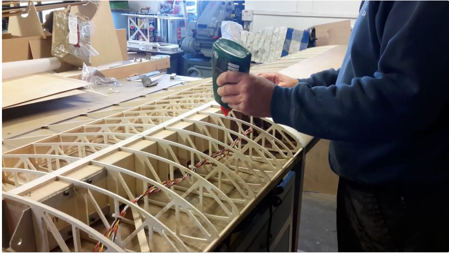
2 - Applying the glue safely to the wing and panel
