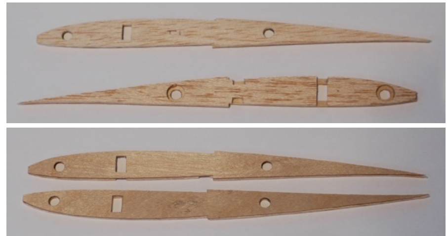
Figure W5: Dihedral break ribs
