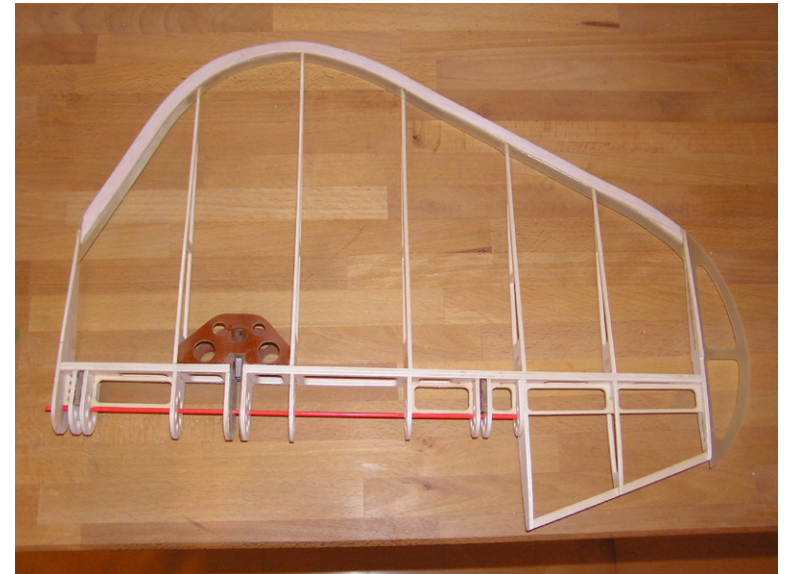
Rudder with the drive element in construction
