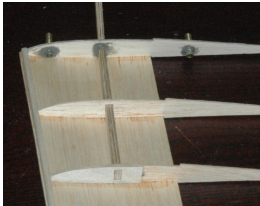
Figure W22: Installing the spar joiner and first three ribs
