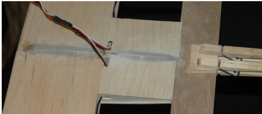
Figure F7: Rear wing mount clamped with clothes pins
