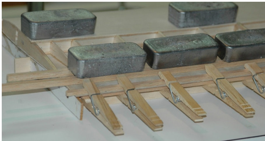
Figure W9: Clamping the trailing edge top skin
