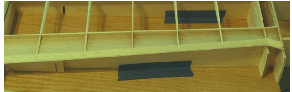
Figure W7: Trailing edge construction
