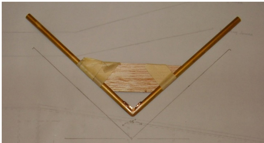
Figure T6: Tail pivot tube assembly template
