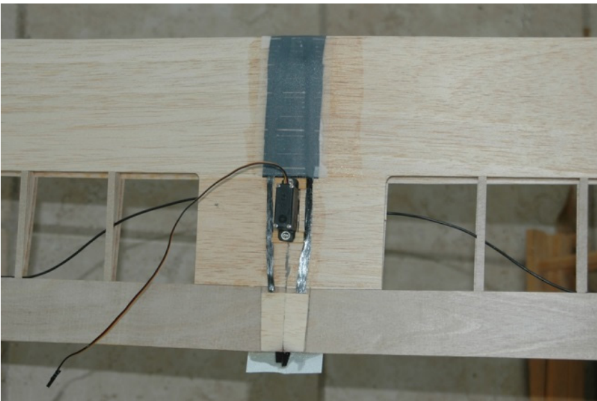
Figure F10: Bottom side of the wing with unidirectional carbon reinforcement being applied.
