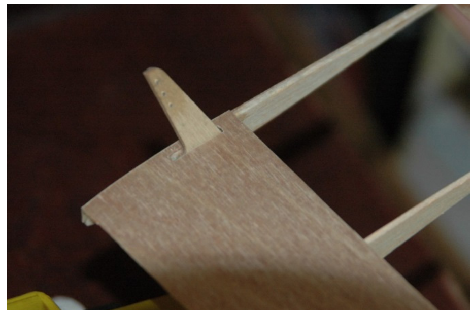
Figure T4: installed control horn
