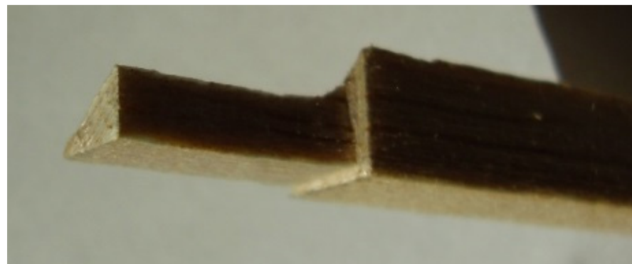
Figure F1: Upper tailboom corner brace shaping detail
