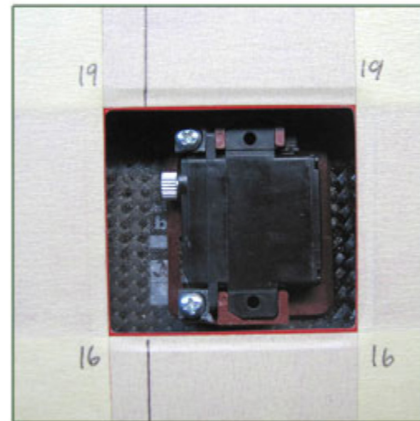
Test fit the servo you want to use; here is one with optional servo frame. If there is sufficient depth, reinforce the inside surface of the servo pocket. The line marks the plane in which the linkage will be located.
