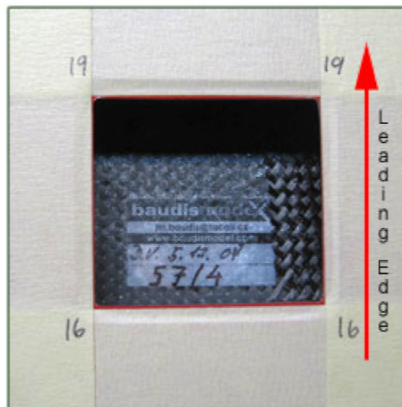
A typical wing-servo pocket in a hollow-molded wing. Tape it off with masking tape to protect the wing and optionally note pocket depth in the corners.
