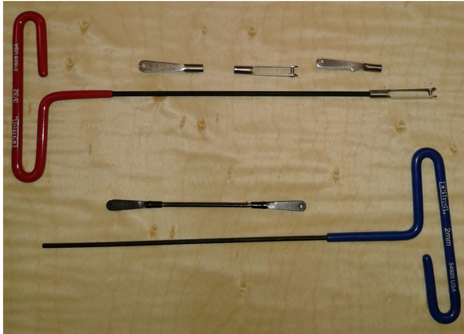
A 3/32" hex wrench works for 4-40 clevises and a 2 mm works for my 2-56 clevises.
