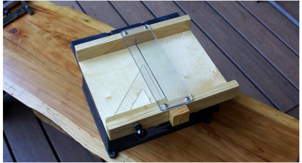
Bill Wilson's cross-cut sled.
