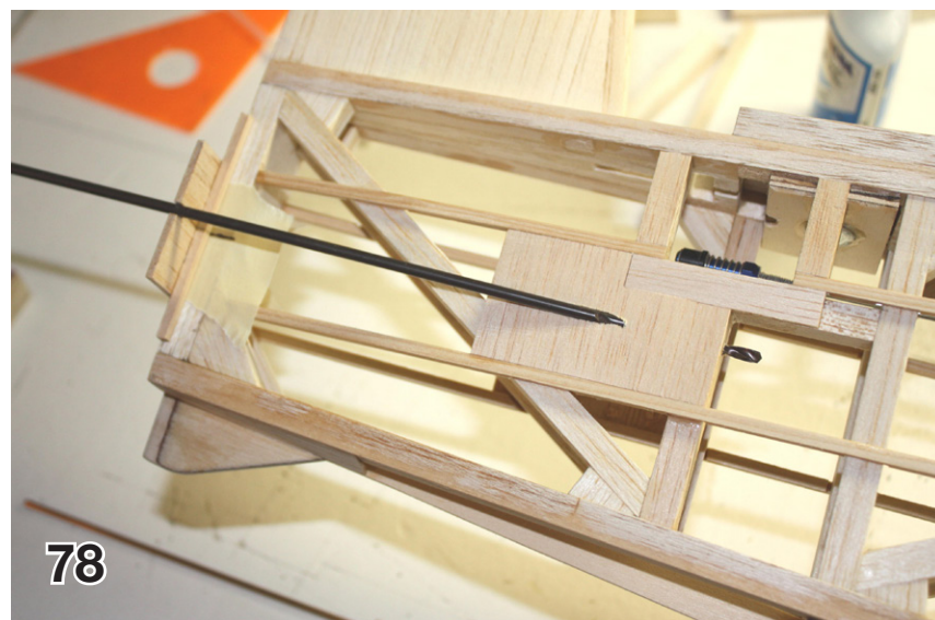
77 & 78. Use a small jig to get the angled hole correctly located and accurate. The hole is drilled with a piece of sharpened 1/8" O.D. brass tube.
