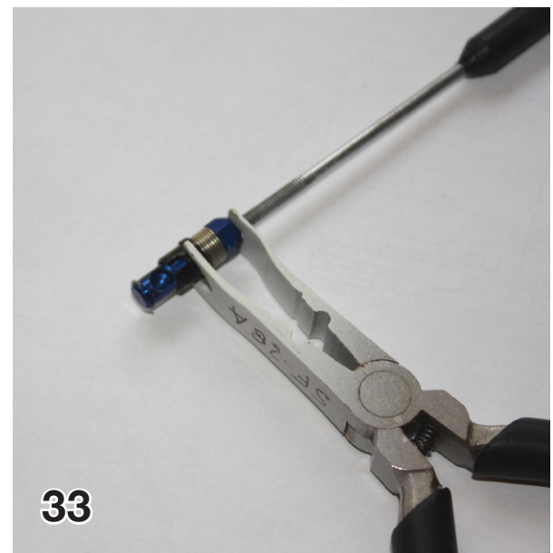
32 & 33. Modified helicopter ball link pliers are used to retract the sleeve and release the ball.
