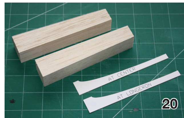
20. Rough-cut blocks and templates.
