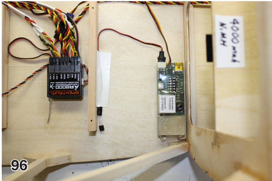
96. Sky Assistant vario/telemetry unit mounted against aft side of former F3.
