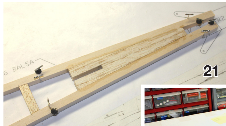
21. The fill-in between the aft upper longerons is made from four pieces of 5/16" sq. balsa edge glued and cut/sanded to fit.
