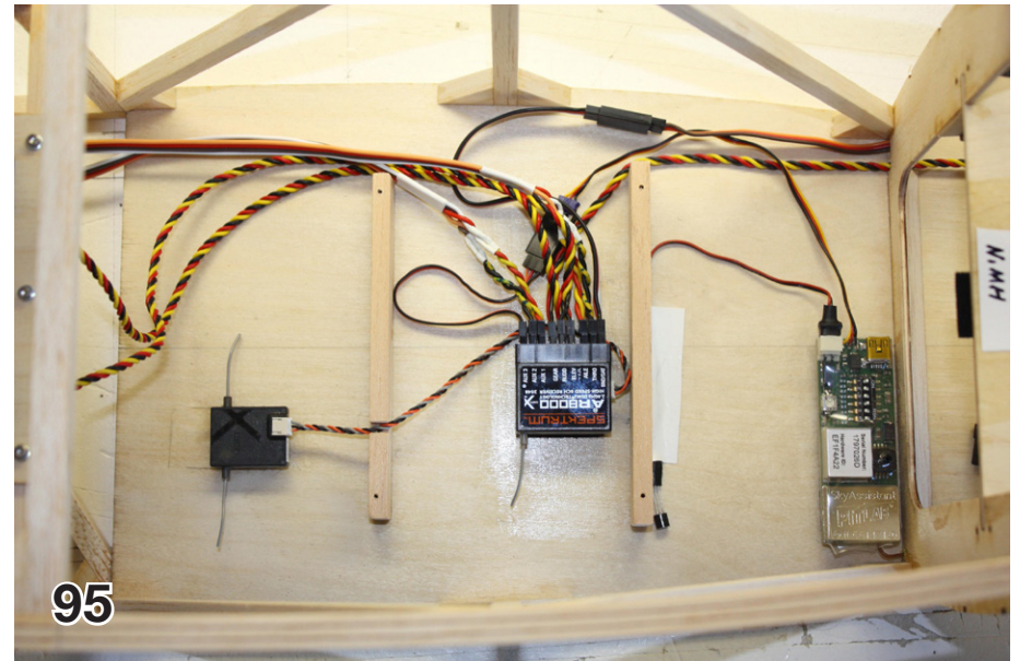
95. An overhead shot of all the various wires hooked to the receiver. See text for placement of additional satellite receivers on the fuselage sides.
