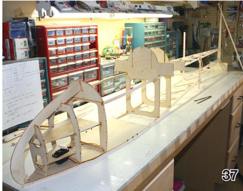
37. Upper longerons, fin post, and formers F6 and F7 jugged for gluing.
