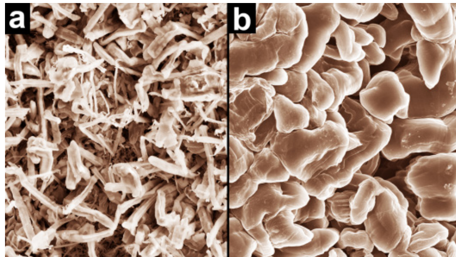
Scanning electron microscope images that show how normal electrolyte promotes dendrite growth (a, left), while PNNL's new electrolyte produces smooth nodules that don't short-circuit cells (b, right)
