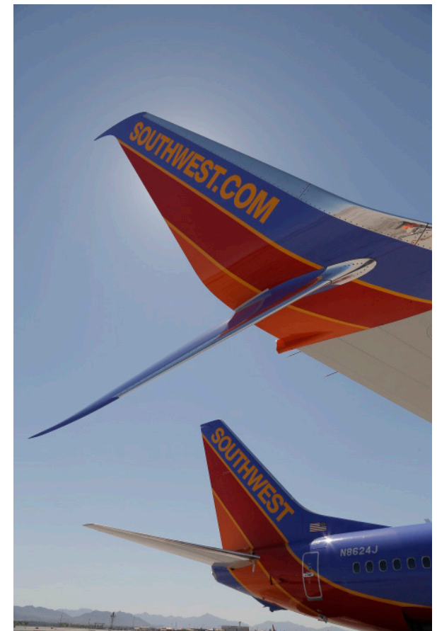
Retrofitting Blended Winglets to Split Scimitars involves adding strengthening spars, aerodynamic “scimitar tips,” and a large ventral strake.
