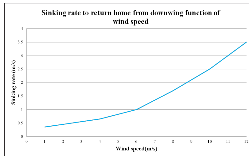
Figure 11: If a plane can return home flying “as usual” in a light wind condition, in strong wind, the plane must “dive”. That’s not easy to do and need lots of practices in such heavy conditions.
