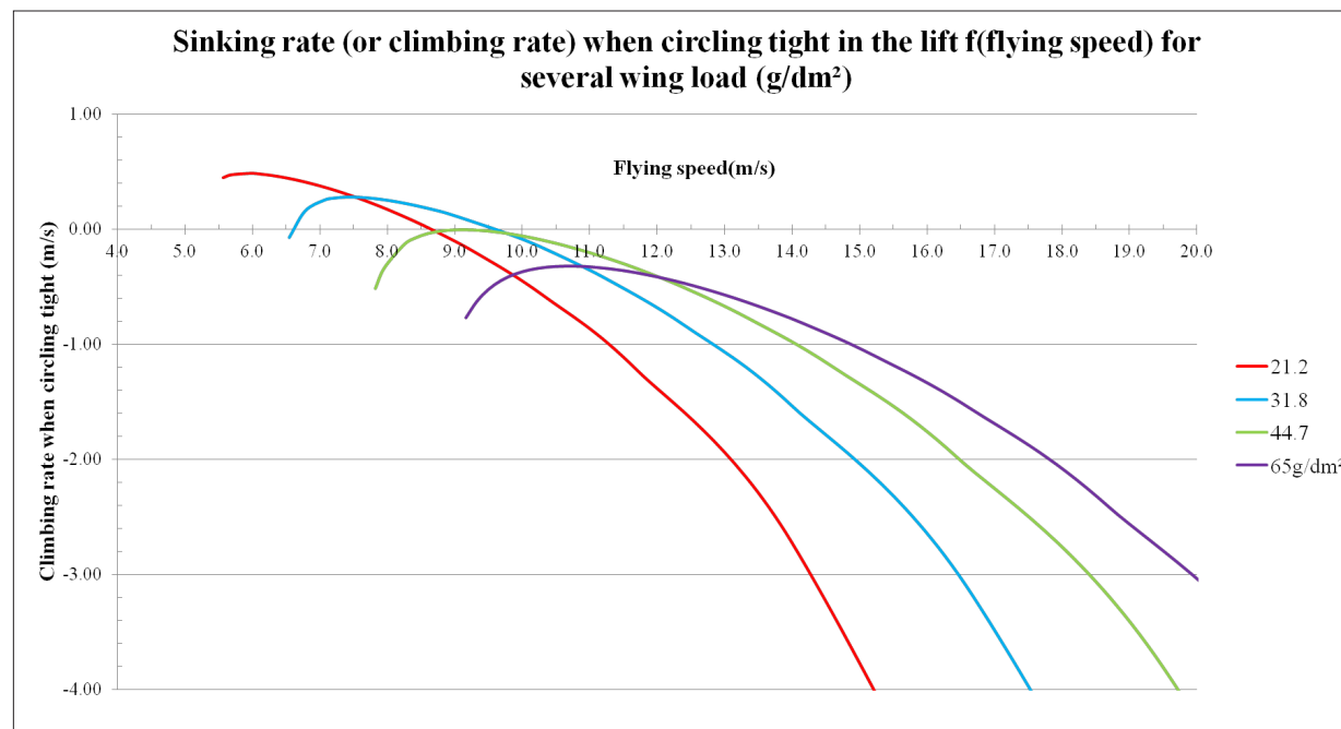
Figure 7: Example of a plane circling in the same thermal when more or less ballasted. It may take the lift or sink...
