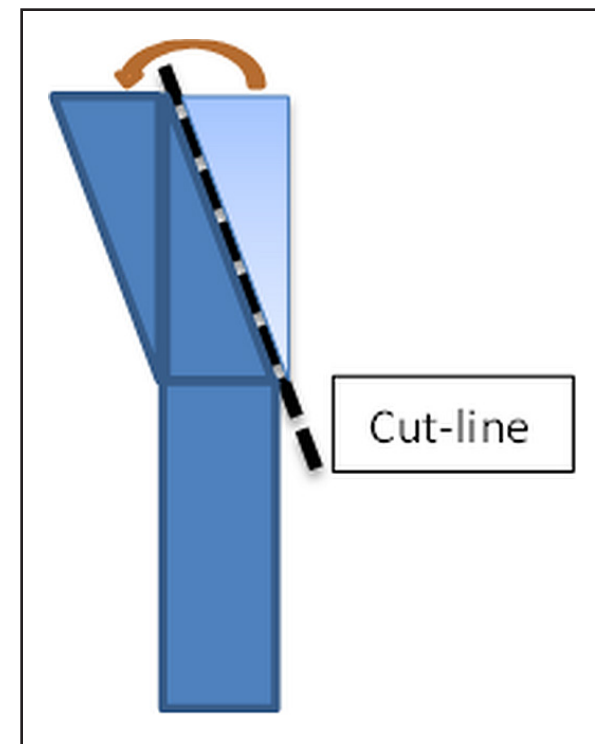
Basic main spar construction. See text for details.
