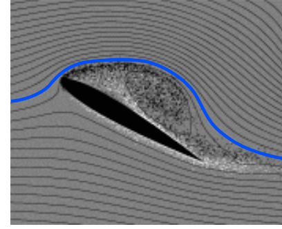
Figure 2: Simulations by Leon van Dommelen, Ph.D. Comments and colored arrows by P. Randolph
