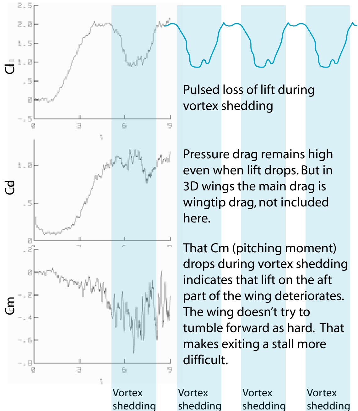
Figure 3: C_l , C_d , C_m
