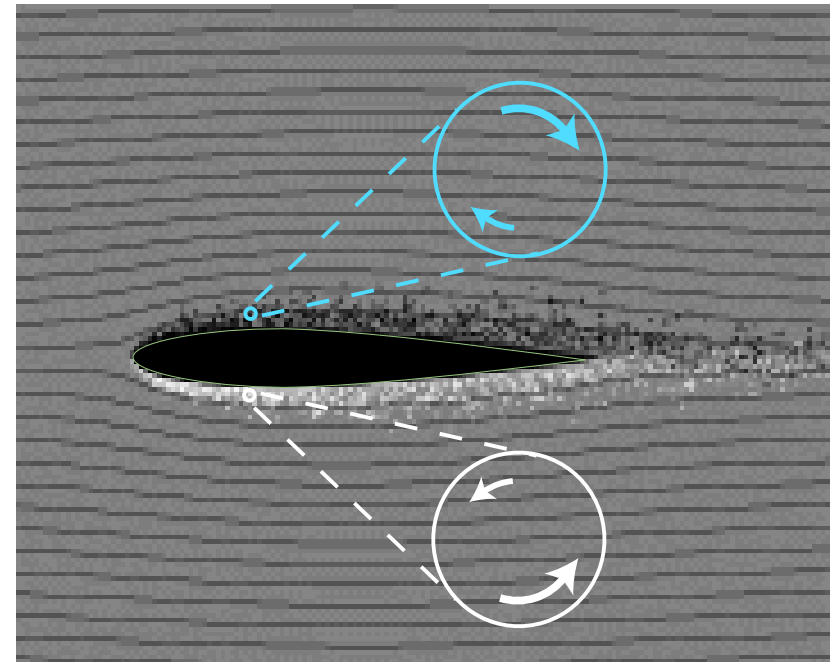
Figure 4: T = 1.00 of Dr. Dommelen's simulation series. Dr. Dommelen writes, "In the simulation, the boundary layer is represented as vortices (miniature tornadoes, which are displayed as black or white dots, depending on direction of rotation.)"
