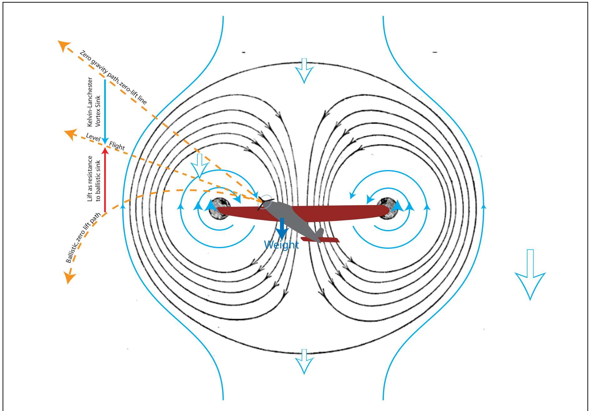
Figure 9: Kelvin's diagram (in black) of a traveling vortex (sinking, here), illustrating Lanchester's vortex sink flows. © 2011 Philip Randolph
