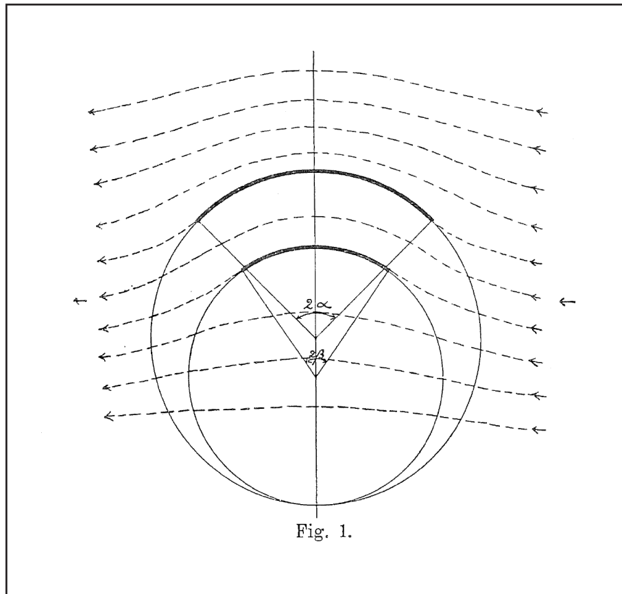
Figure 6: Wilhelm Kutta's 1902 diagram of the lift of a thin, arc wing. With mathematics divorced from concept, he neither recognized waveform nor circulation around a wing, and yet applied a 'circulation' factor to define his flows
