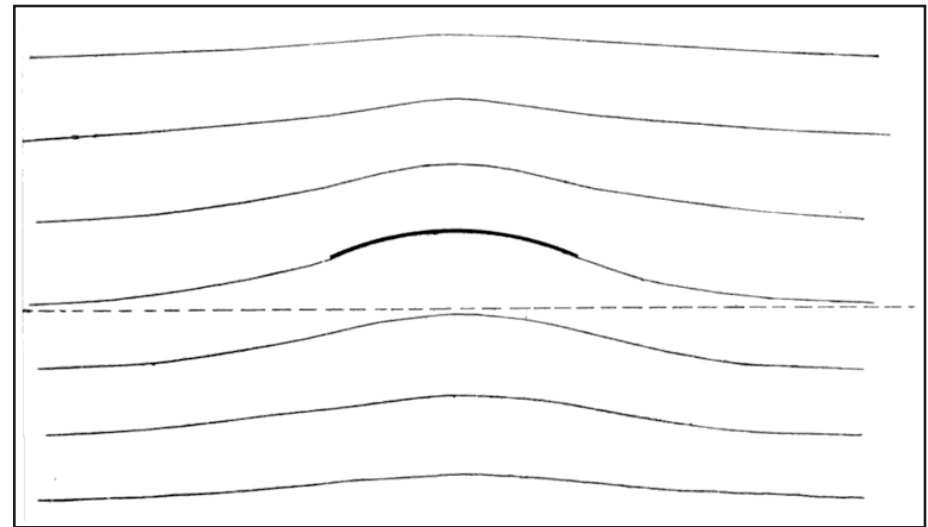
Figure 1: Lanchester’s ‘supporting wave’ diagram, used in his 1894 presentation. He only applied such symmetry and perfect lift to infinitely long wings in inviscid (frictionless), incompressible fluids. The airfoil was curved to match the path of air, to avoid ‘discontinuities’ at leading and trailing edges, a requirement later known as the ‘Kutta condition.’ Flows over a subsonic wing in lift always show waveform, with upwash ahead rising to a crest, and downwash behind. © 2011 Philip Randolph
