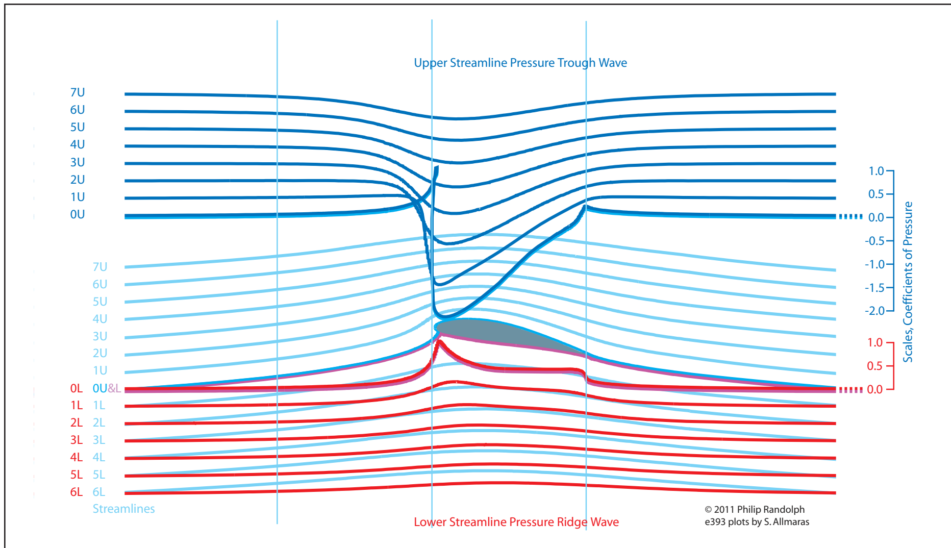
Figure 22: Upper and lower pressure waves along streamlines. Energy in springs is stored either by compression or stretch. Waves along a spring are an exchange of momentum for tension or compression. It's the same for pressure gradients — raised or lowered, they store energy, that around a wing is temporarily exchanged for velocity of air, kinetic energy. Such energy patterns are 'carried along' in constant relation to the
