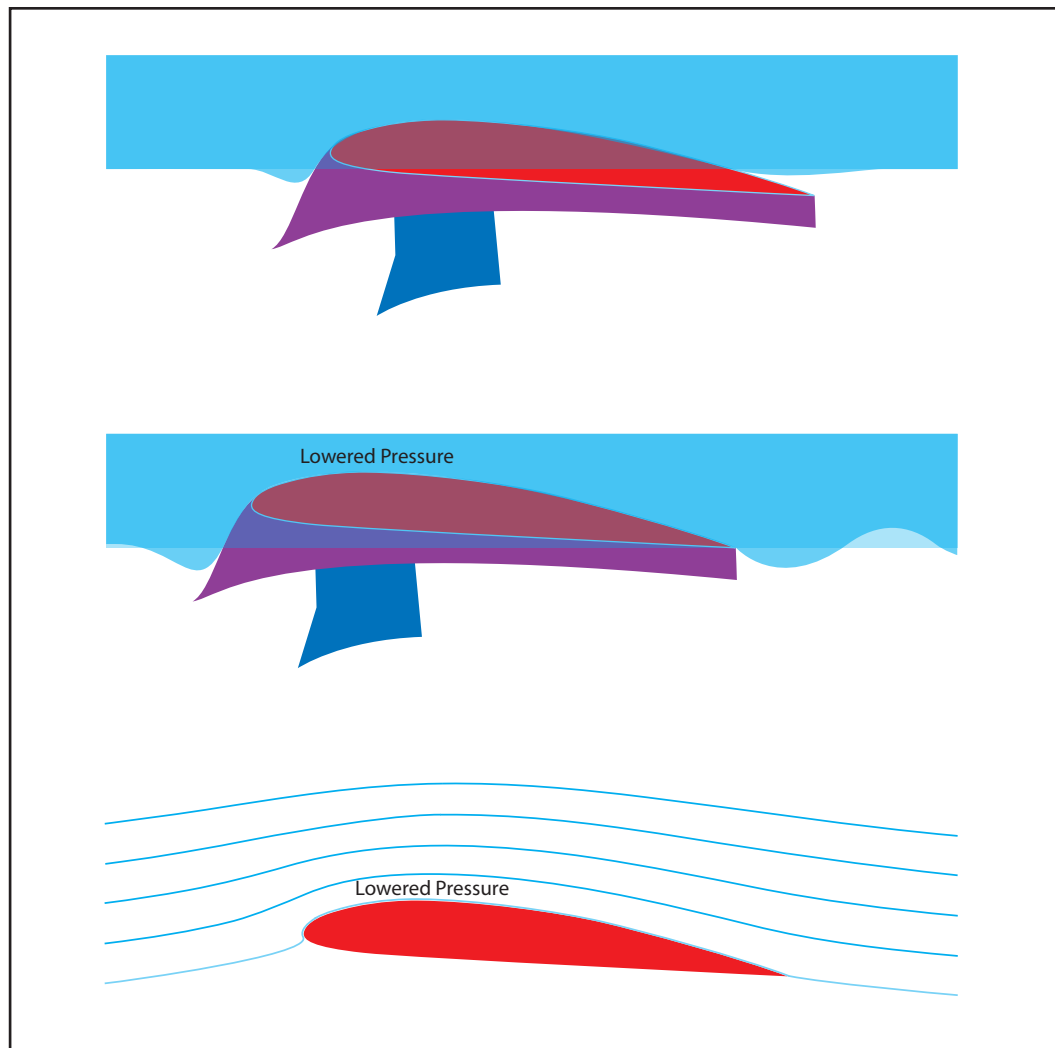
Figure 24: Airfoil boat. Displacement hulls and buoys lift downwards in the same way Russell's 'negative solitary wave' lowers pressure on a wing's upper surface. As a displacement boat hull picks up speed, it centrifuges a lowered pressure beneath it and 'lifts' down into water in the same way a wing centrifuges a lowered pressure above it, and lifts, up. The negative lift on a hull (lowered pressures) is in balance with buoyancy and weight. The lift on a wing is the difference between lowered pressures above and less-changed pressures below. © 2011 Philip Randolph
