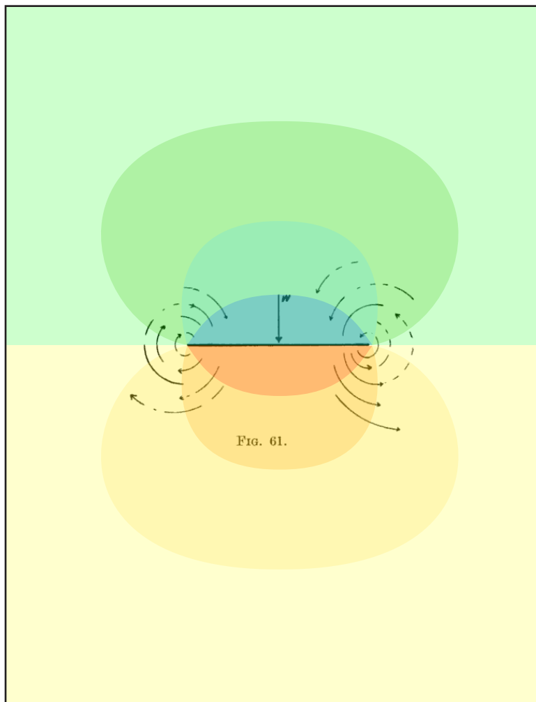
Figure 10: The equivalence of Lanchester's 'acceleration fields' and pressure gradient forces. Lanchester's early diagram (in black) of a vertically sinking, flat plate. Superimposed are pressures (not to scale). Lanchester's 'acceleration field' arrows show the pressure gradient forces from highest pressures below (red) to lowest pressures above (blue), that slow the plate's sink.
