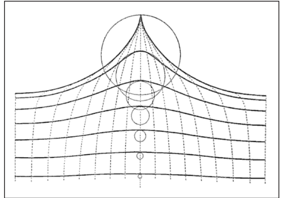
Figure 3: Horace Lamb's 1895 interpretation of von Gerstner's 1802 deep-water wave-circulation diagram As a wave passes, the water that makes it up moves in complete circles, that diminish with depth.
