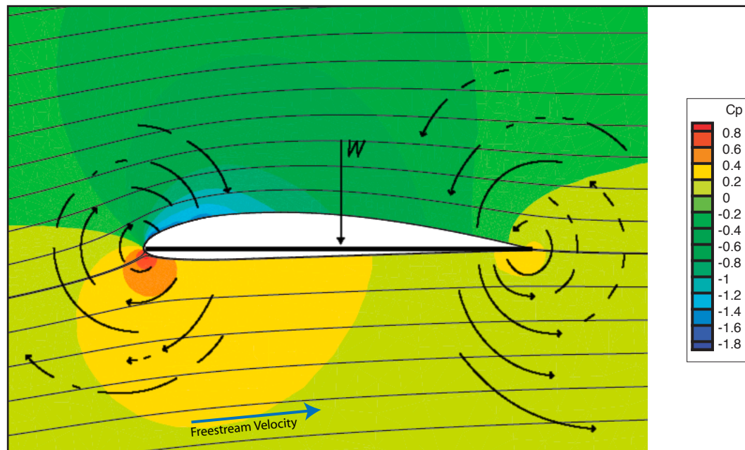
Figure 11: Lanchester figured his 'acceleration fields' would persist even as his flat plate 'flew' forward and down, approximately true. A reproduction of Lanchester's early diagram of a gliding, flat plate and 'acceleration fields' (black) is superimposed on a pressure 'isoline' plot around a modern airfoil. Lowest pressures are in cool colors, highest pressures in warm colors. Pressure gradient forces are at right angles to pressure 'isolines,' lines of constant pressure. Lanchester's diagram is qualitatively accurate. It also shows the forces that create upwash ahead and slow downwash aft.
