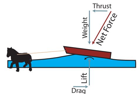
Figure 17: Flow similarity: Dissimilar forces in similar patterns make similar wave motions. © 2011 Philip Randolph
