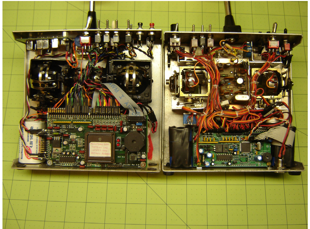
The ProLine is on the right while the original MicroStar 2000 radio is on the left. The latest version of the M*2K encoder is considerably smaller than the hand wired unit that first was produced.
