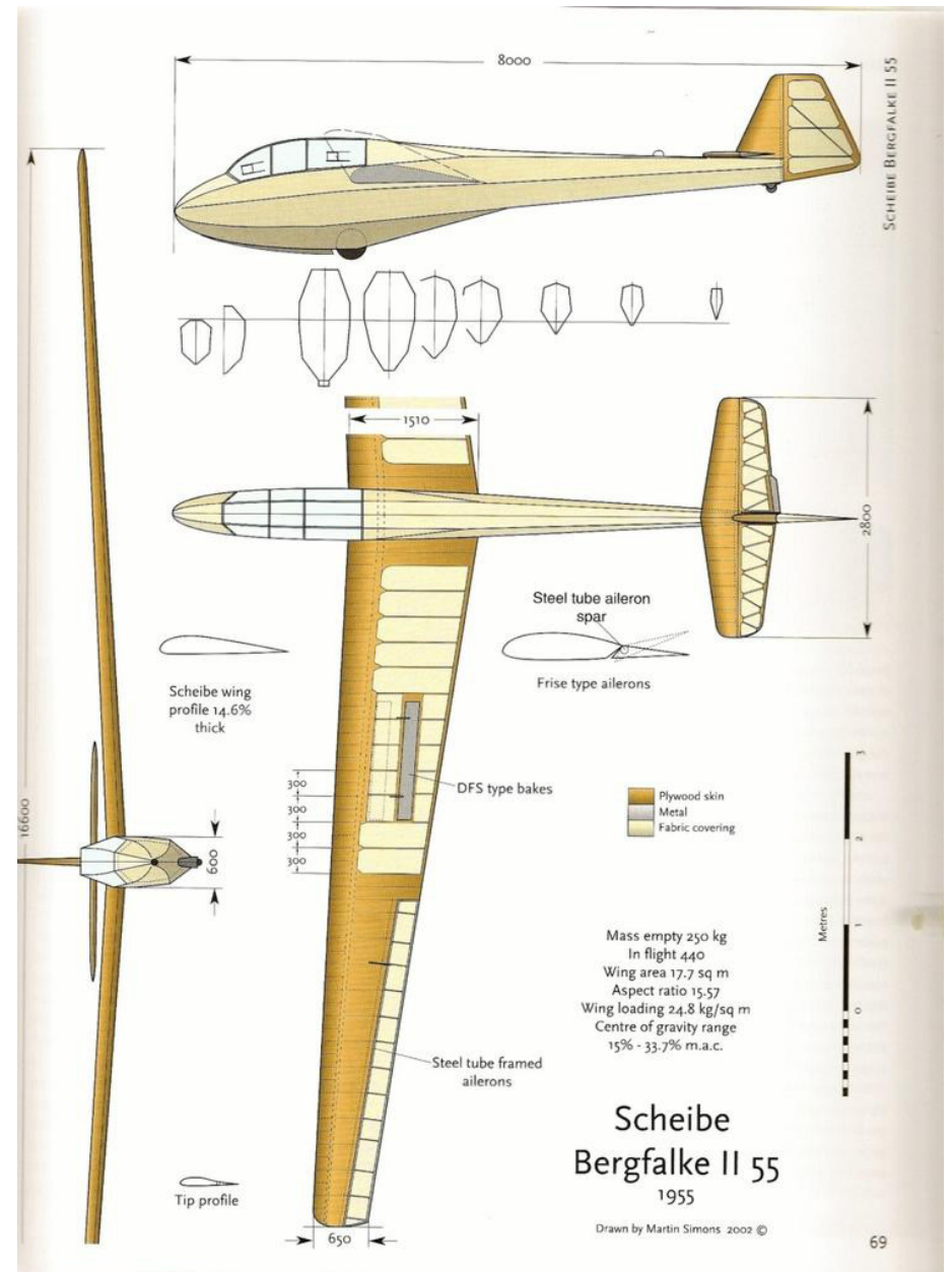
Scheibe Bergfalke II 55 3-view from Sailplanes 1945-1965 by Martin Simons © 2006, published by EQIP <www.eqip.de>. Used with permission.
