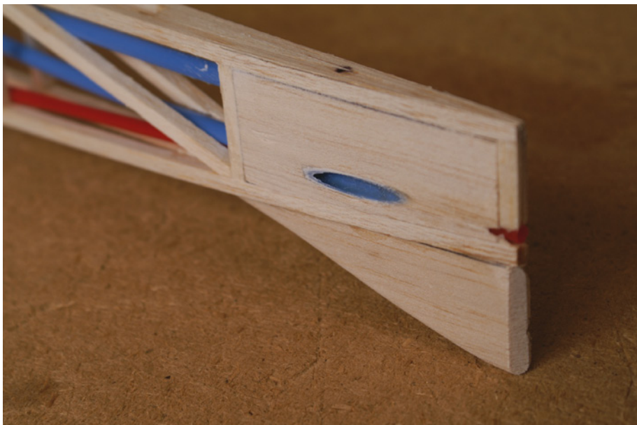
The rudder pushrod exits the left side of the fuselage, the elevator pushrod exits on the right. Notice the red “soda straw” antenna tube at the bottom of the fuselage. The antenna is threaded through this tube and hangs free from the rudder hinge line.
